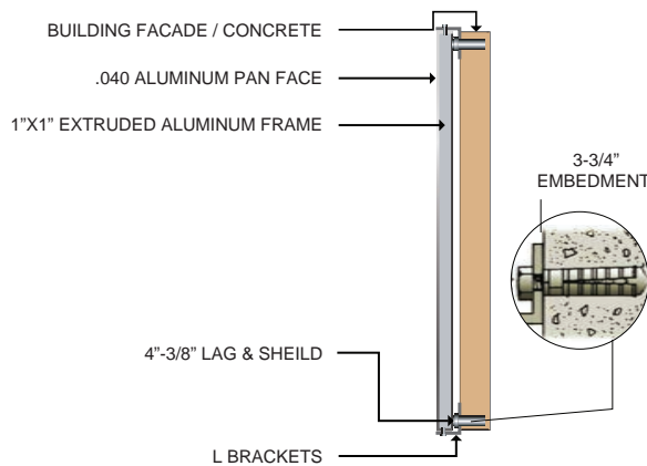
MOUNTING DETAIL
